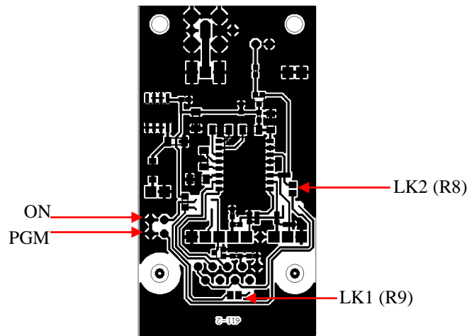
Figure 3: PCB layout of TDi2 (bottom view)
