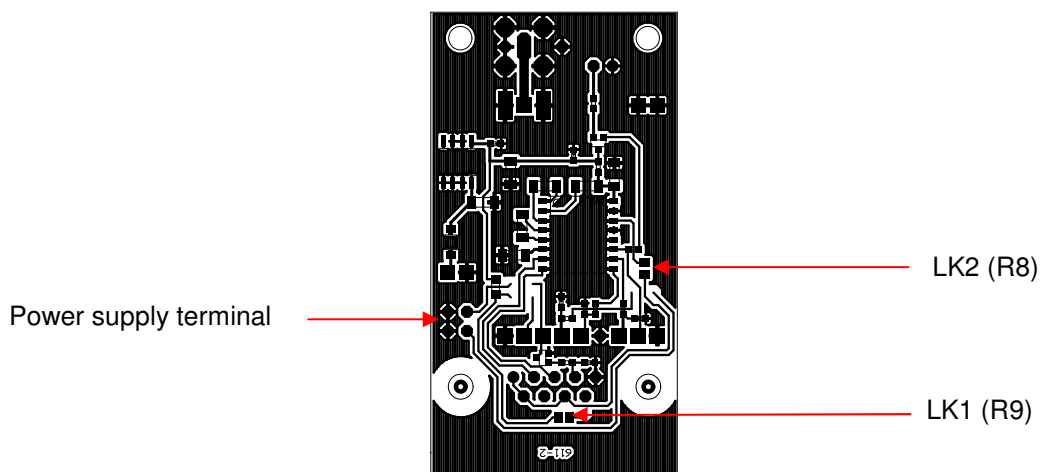
Figure 3: PCB layout of TDi2 (bottom view)
