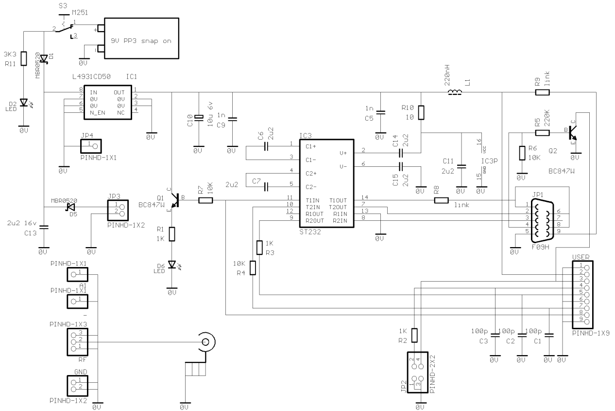
Figure 2: Schematic diagram of TDi2
