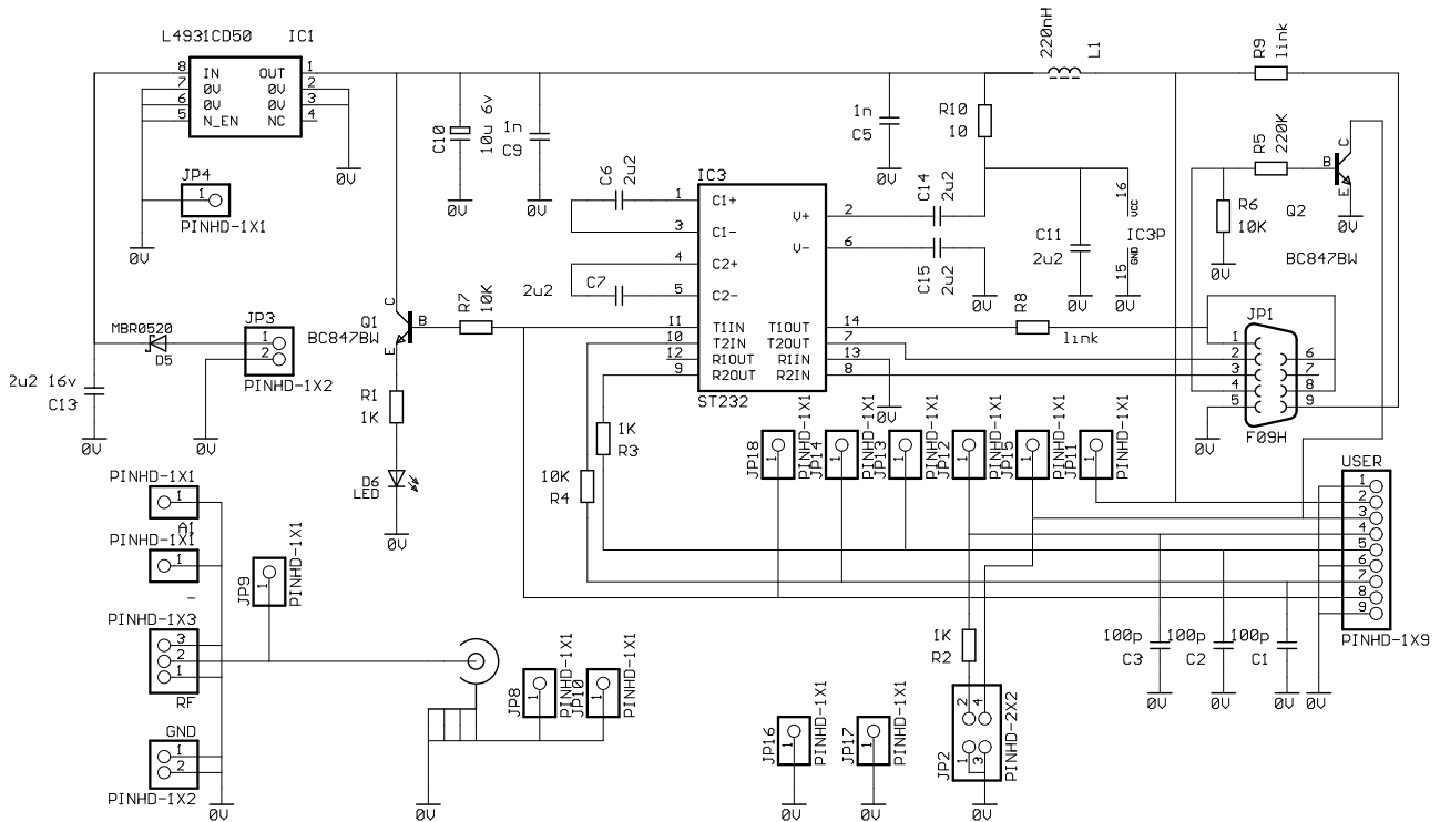
Figure 2: Schematic diagram of TDi2
