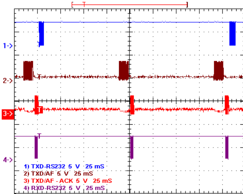
Figure 10: RPM3B operating in slots throughput mode with ACK for each transmission
