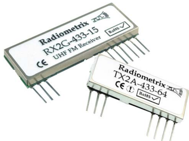
Figure 1: RX2G-433-15 & TX2A-433-64
